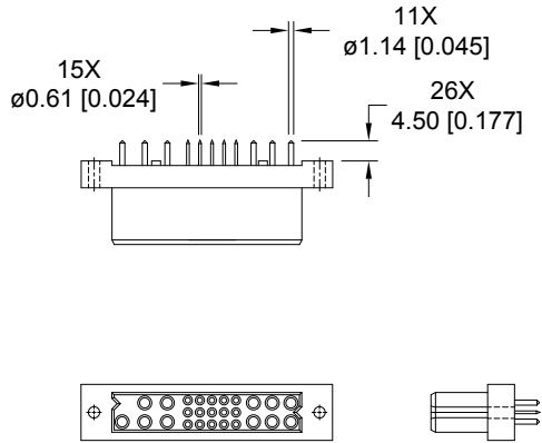
CONNECTOR DIMENSIONS
