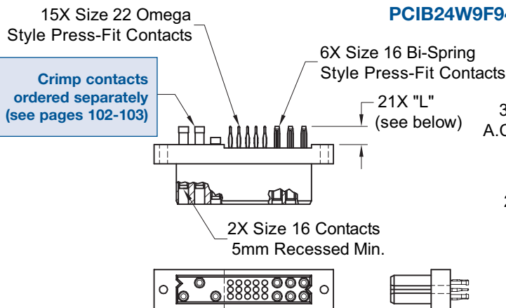
CONNECTOR DIMENSIONS
