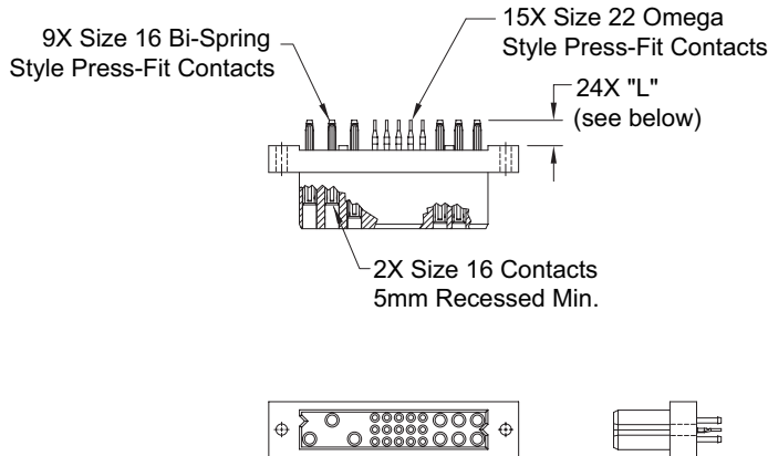
CONNECTOR DIMENSIONS
