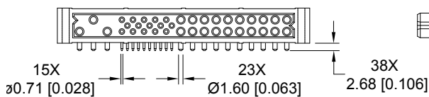
CONNECTOR DIMENSIONS
