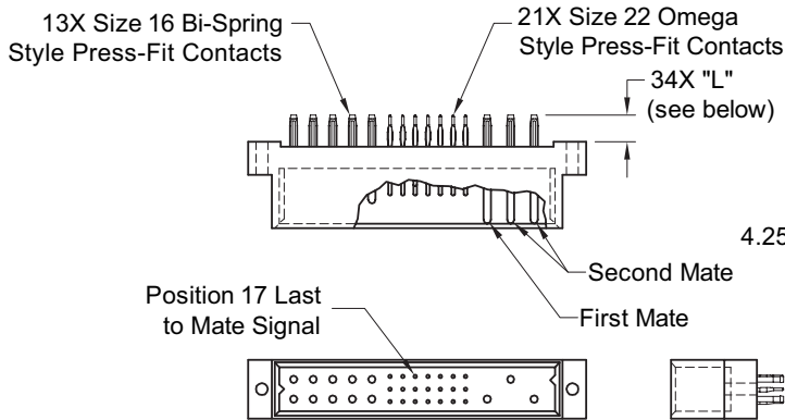
CONNECTOR DIMENSIONS
