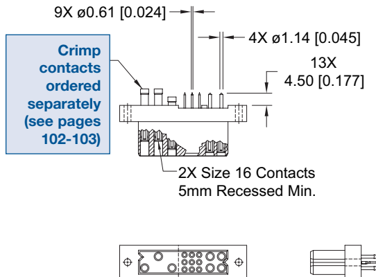
CONNECTOR DIMENSIONS
