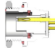
#16 Contacts for HS3 and TS3 Series
