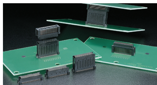
Micro Stack
